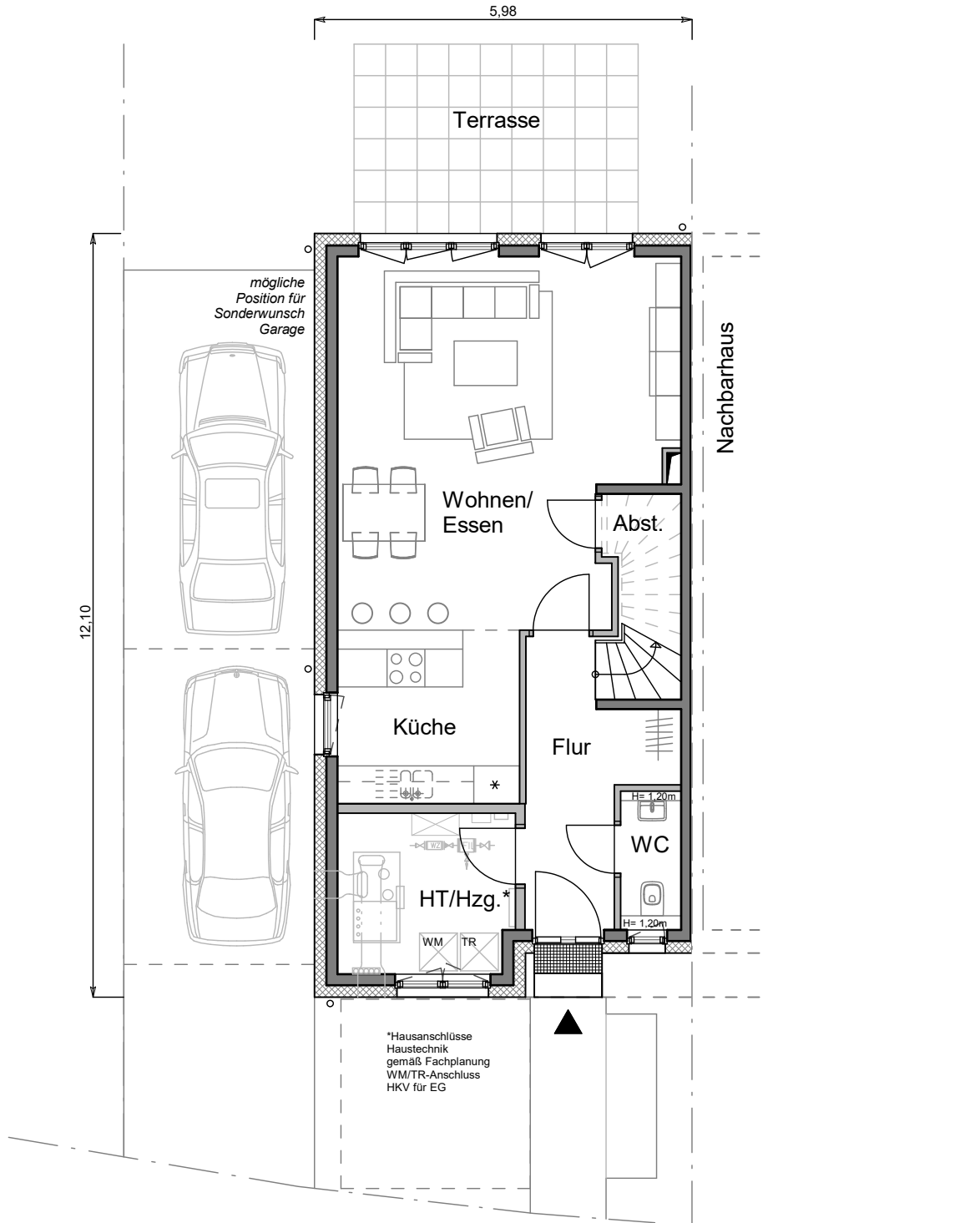
ERDGESCHOSS M 1:100/DIN A4
